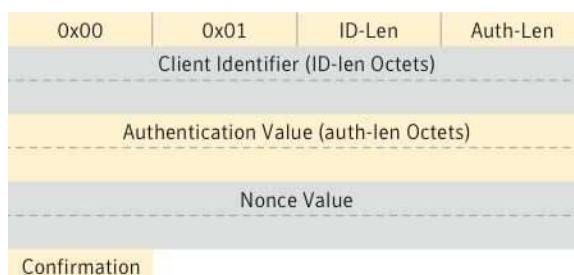
Fig. 37. The general format of the authentication data. In secure qualification, this data is positioned after the UDP header.
