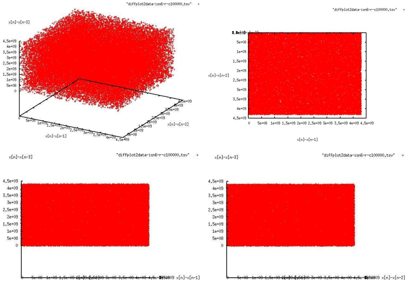
Fig. 47. Plot of \langle x[n]-x[n-1], x[n]-x[n-2], x[n]-x[n-3] \rangle for each of 100,000 ISNs in response to IPv6 TCP SYN requests with randomly generated source ports. The view at an angle and head-on from three different non-parallel sides.
